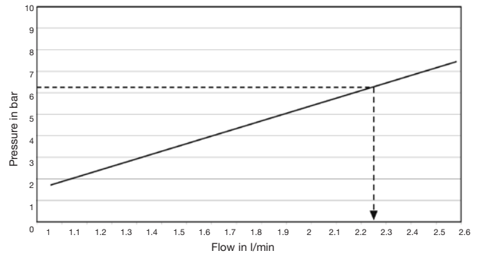
Flow characteristics OFF-LINE Filter OLS with filter element SRM-30HB (at maximum viscosity)
