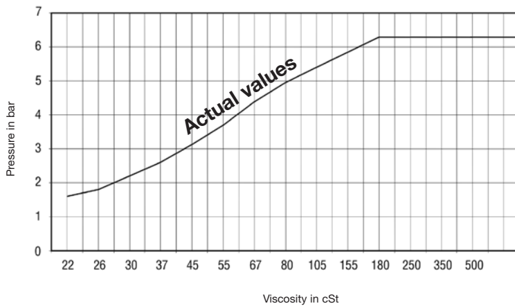
Filter element SRM-30HB \Delta p / viscosity - graph (at a flow of 2.1 l/min (0.6 US GPM) per element)
